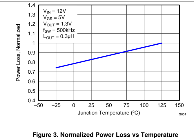
Figure 3. Normalized Power Loss vs Temperature
