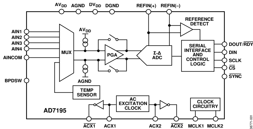
Figure 18. Block Diagram
