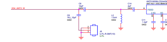
Figure 13. Schematic
