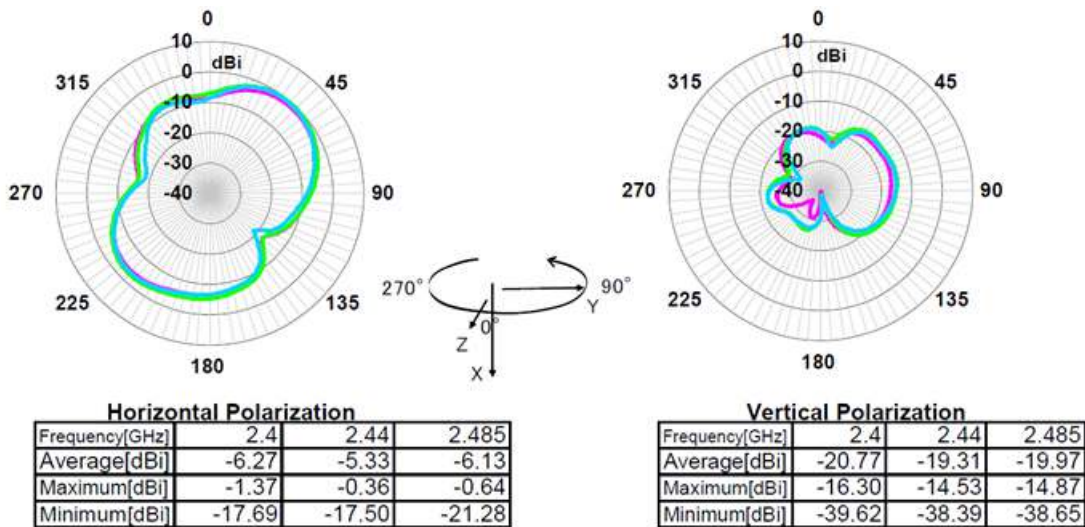
Figure 8. ANT1 Polarization
