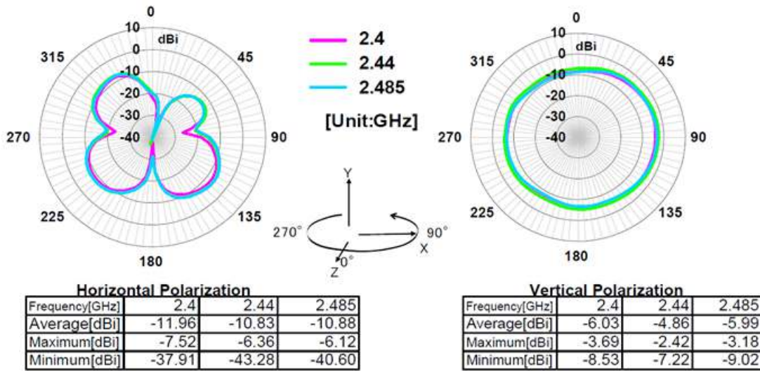
Figure 7. ANT1 Polarization
