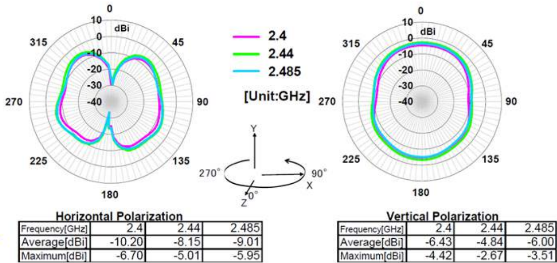
Figure 10. ANT2 Polarization
