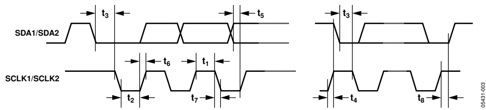
Figure 2. I²C Timing
