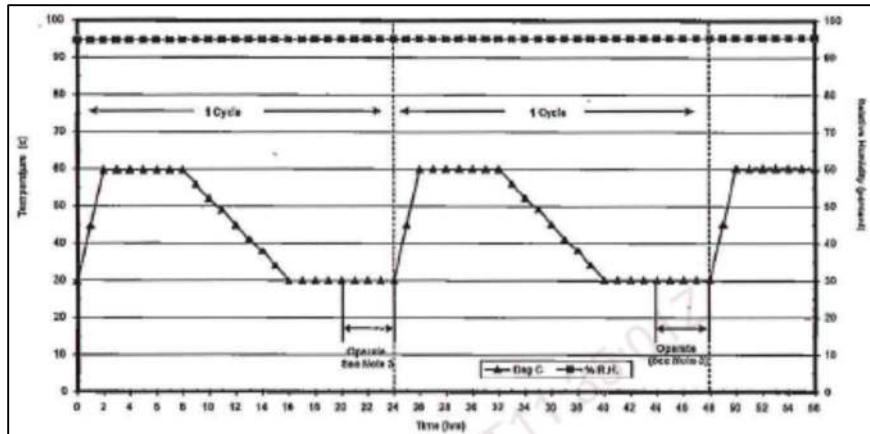
Figure 2 – Humidity Test Chamber Profile
