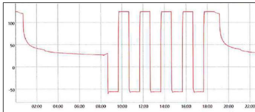
Figure 1 – Thermal Shock Test Chamber Profile
