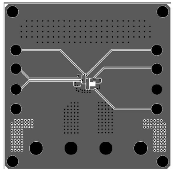
Figure 4: Bottom Layer
