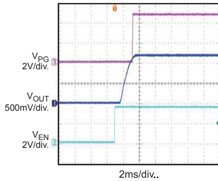
Power Good
