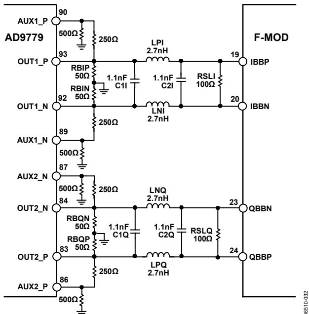
Figure 31. DAC Modulator Interface with Auxiliary DAC Resistors
