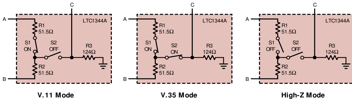
Figure 3. LTC1344A Modes
