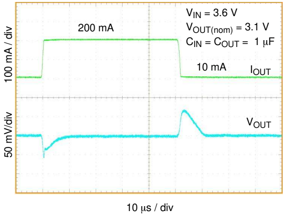
Figure 55. Load Transient Response I_{OUT} = 10 \text{ mA to } 200 \text{ mA}, C_{OUT} = 1 \mu\text{F}
