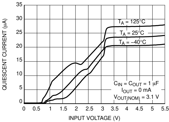
Figure 13. Quiescent Current vs. Input Voltage V_{OUT} = 3.1\text{ V}
