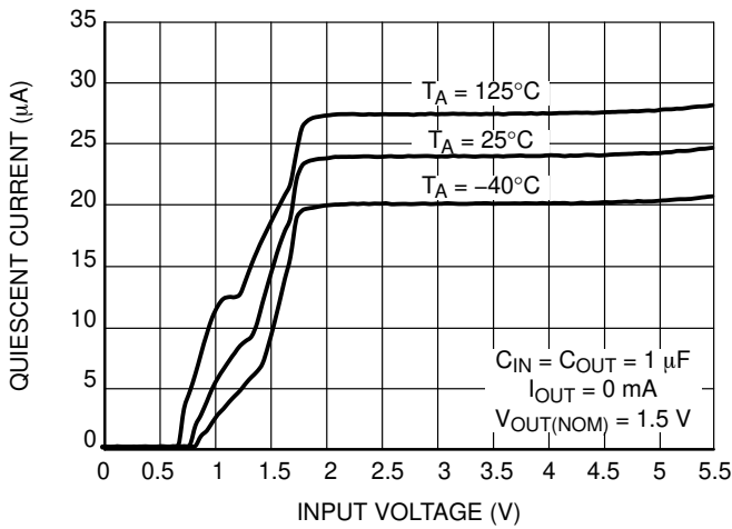
Figure 9. Quiescent Current vs. Input Voltage V_{OUT} = 1.5\text{ V}
