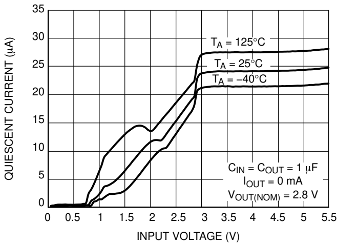
Figure 11. Quiescent Current vs. Input Voltage V_{OUT} = 2.8\text{ V}
