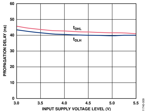
Figure 9. Typical Propagation Delay vs. Input Supply Voltage, V_{DDx}/V_{DDB} = 12 V
