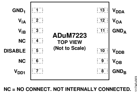
Figure 3. Pin Configuration
