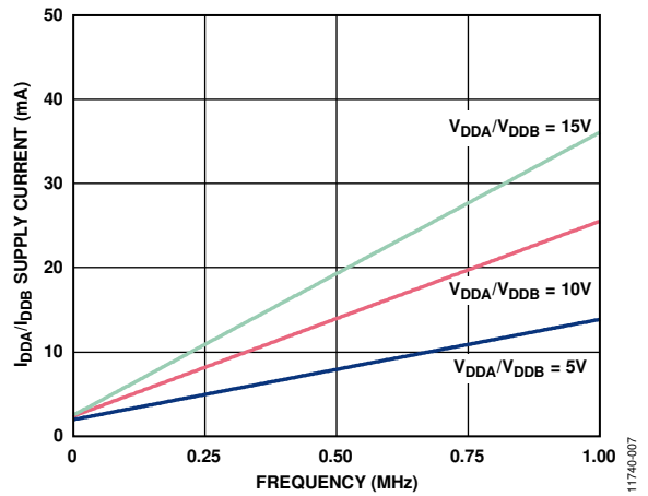
Figure 7. Typical I_{DDx}/I_{DDB} Supply Current vs. Frequency with 2 nF Load
