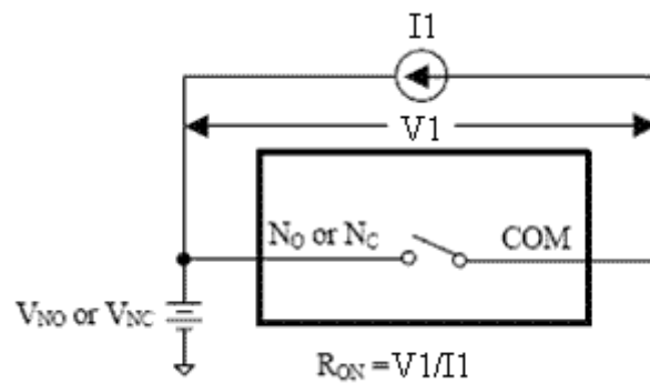
Figure 1, On Resistance
