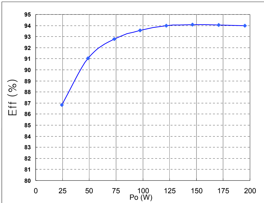
Figure 25. Measured Efficiency
