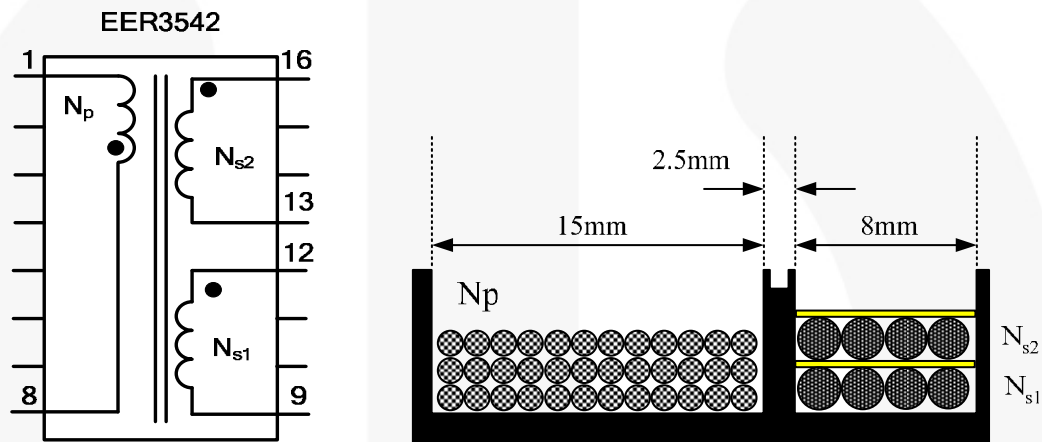
Figure 5. Transformer specification.
