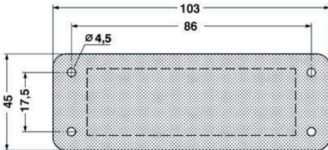
Dimensioned drawing
