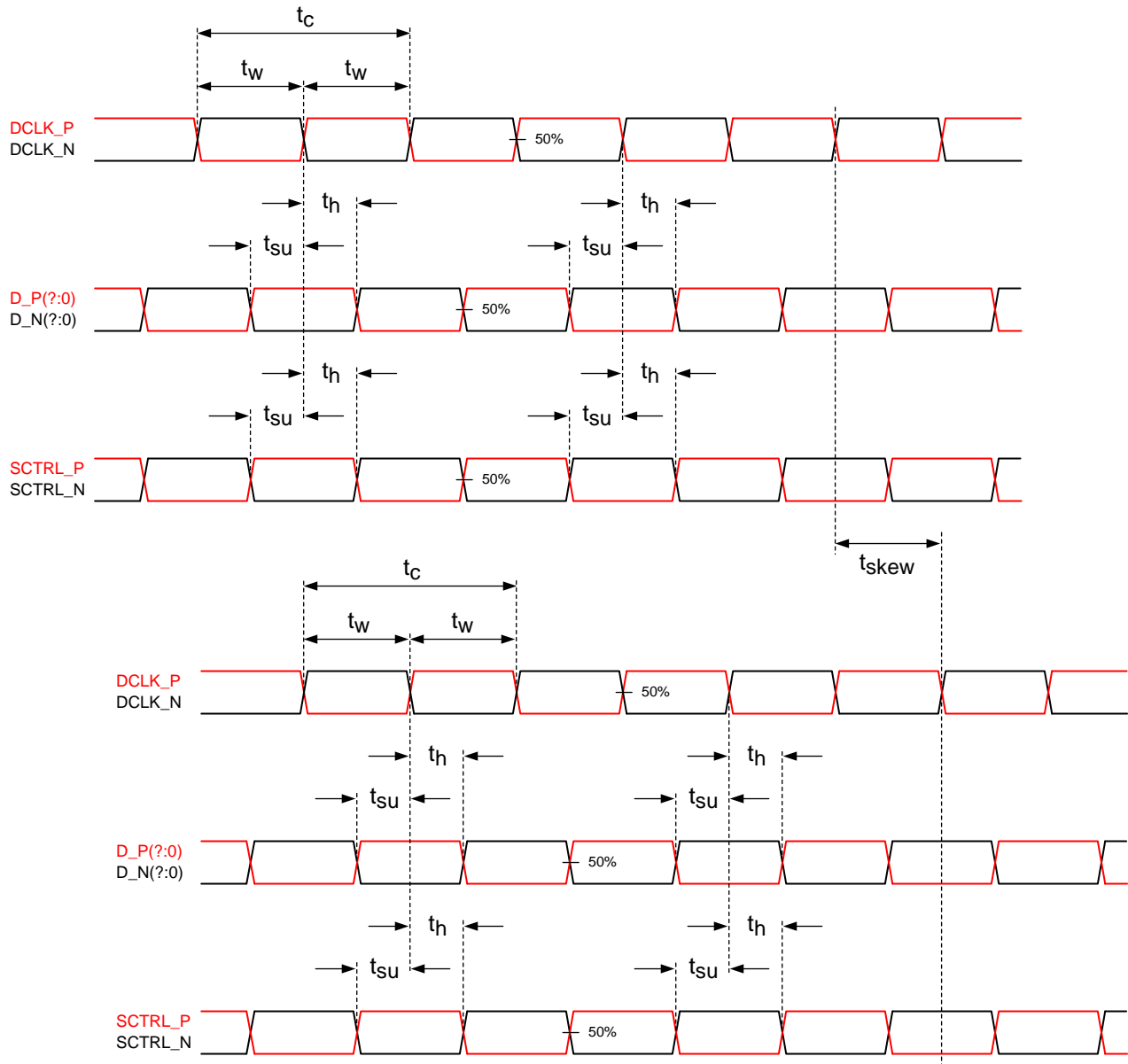
Figure 6. Timing Requirements
