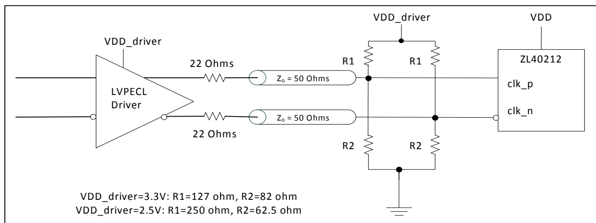
Figure 3 - LVPECL Input DC Coupled Thevenin Equivalent
