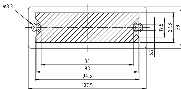
restricted area for Thermal Interface Material
