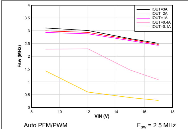
Figure 8-23. Switching Frequency vs Input Voltage V_{OUT} = 5.5\text{ V}
