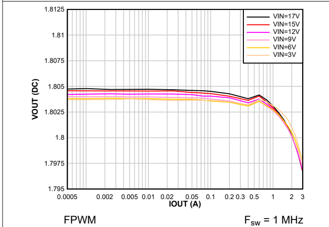
Figure 8-25. Output Voltage vs Output Current V_{OUT} = 1.8\text{ V}
