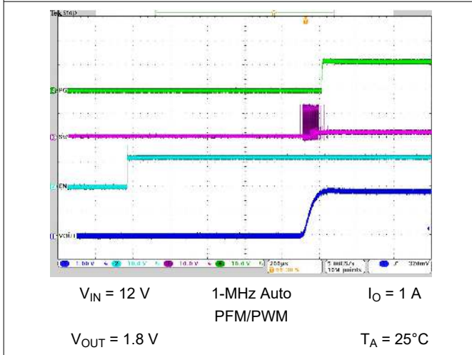
Figure 8-27. Start-Up Timing V_{IN} = 12\text{ V} , V_{OUT} = 1.8\text{ V} , I_{OUT} = 1\text{ A} , T_A = 25^\circ\text{C}
