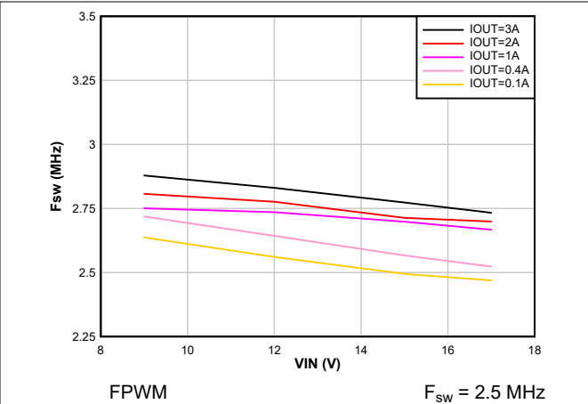
Figure 8-24. Switching Frequency vs Input Voltage V_{OUT} = 5.5\text{ V}
