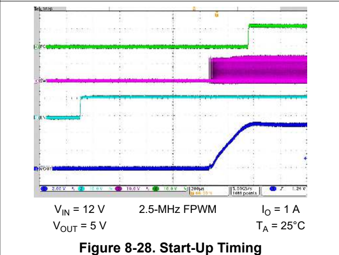
Figure 8-28. Start-Up Timing V_{IN} = 12\text{ V} , V_{OUT} = 5\text{ V} , I_{OUT} = 1\text{ A} , T_A = 25^\circ\text{C}
