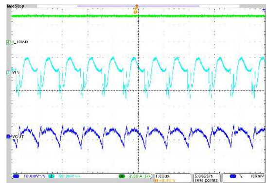
V_{IN} = 12\text{ V} 2.5-MHz Auto I_O = 3\text{ A} PFM/PWM V_{OUT} = 1.2\text{ V} T_A = 25^\circ\text{C}
