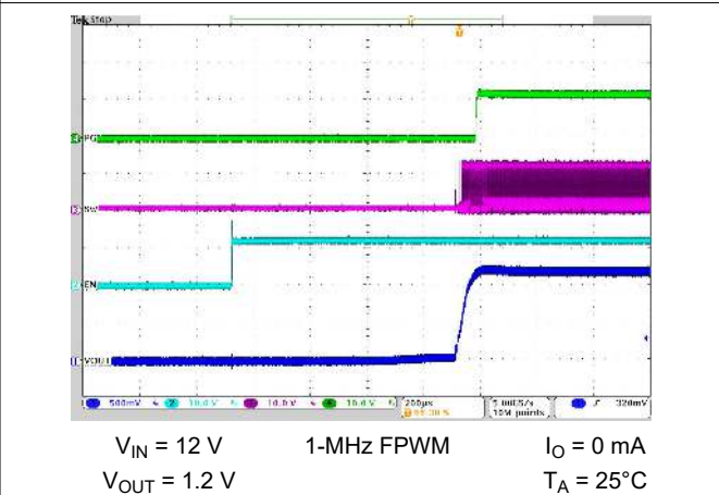
Figure 8-26. Start-Up Timing V_{IN} = 12\text{ V} , V_{OUT} = 1.2\text{ V} , I_{OUT} = 0\text{ mA} , T_A = 25^\circ\text{C}
