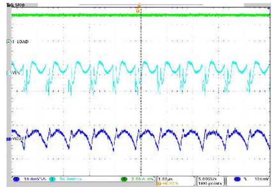
V_{IN} = 12\text{ V} 1-MHz Auto I_O = 3\text{ A} PFM/PWM V_{OUT} = 1.2\text{ V} T_A = 25^\circ\text{C}
