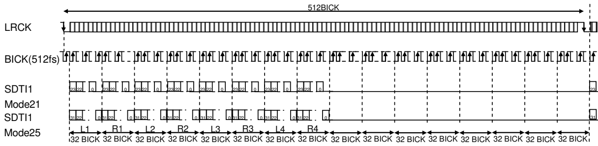
Figure 24. Mode 21/25 Timing
