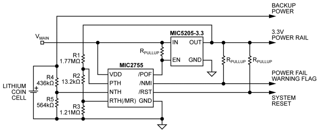
Figure 5. Voltage Supervisor and Backup Battery Monitor
