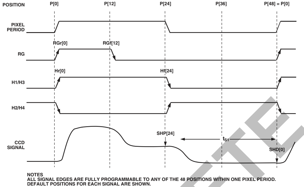
Figure 7. High Speed Timing Default Locations
