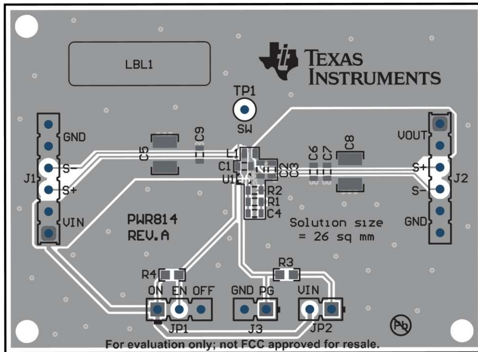
Figure 3. Top Assembly
