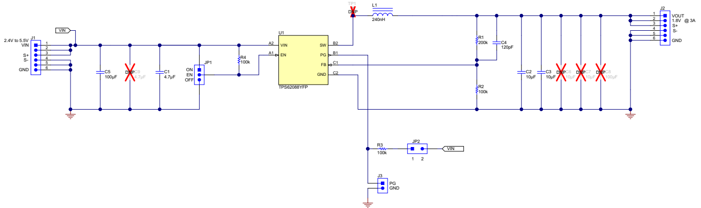
Figure 8. TPS62088EVM-814 Schematic
