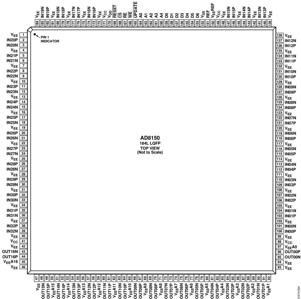
Figure 4. Pin Configuration
