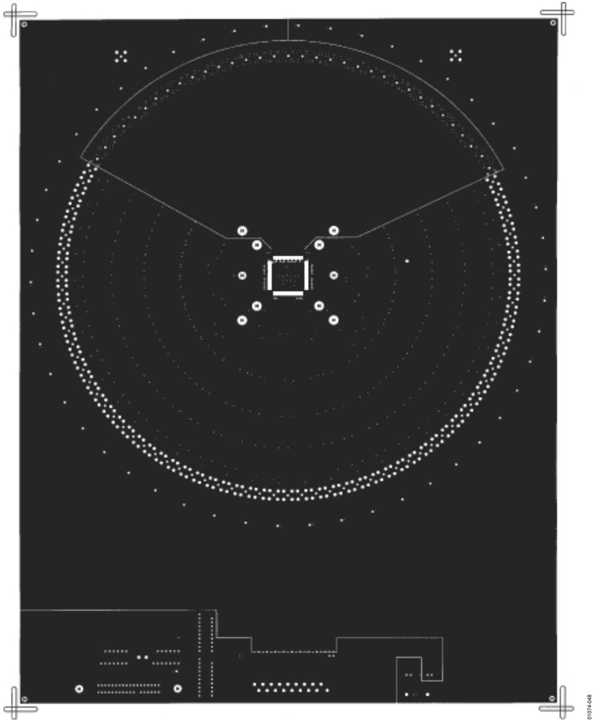
Figure 49. INT1 ( V_{EE} )
