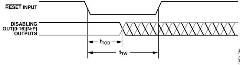
Figure 30, Asynchronous Reset
