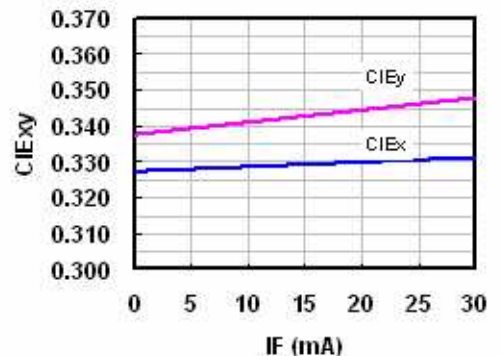
Fig.7. CIE_x vs. Forward Current
