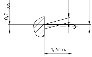
View W 5:1
