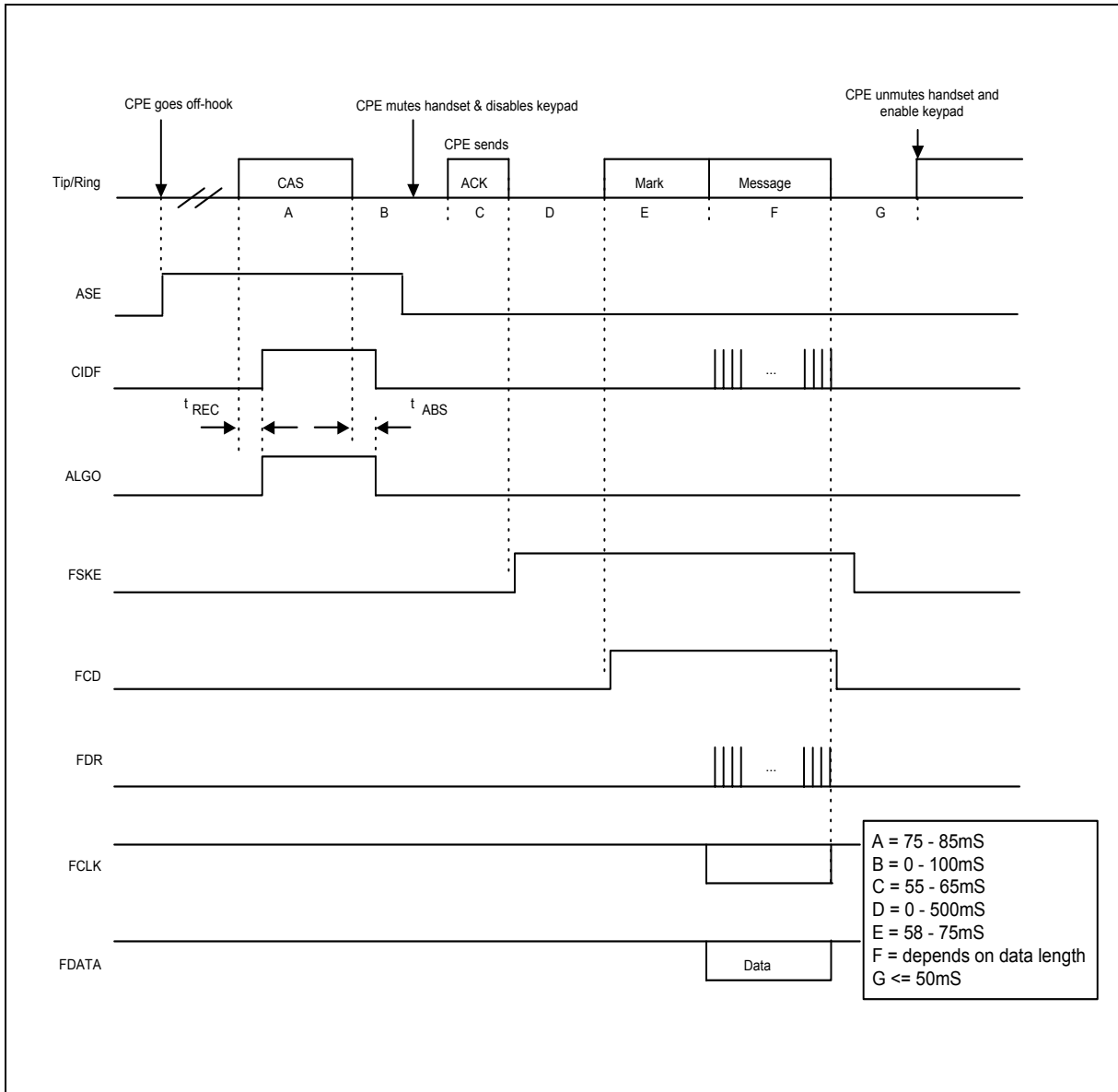
Figure 6-28 Input and Output Timing of Bellcore Off-hook Data Transmission
