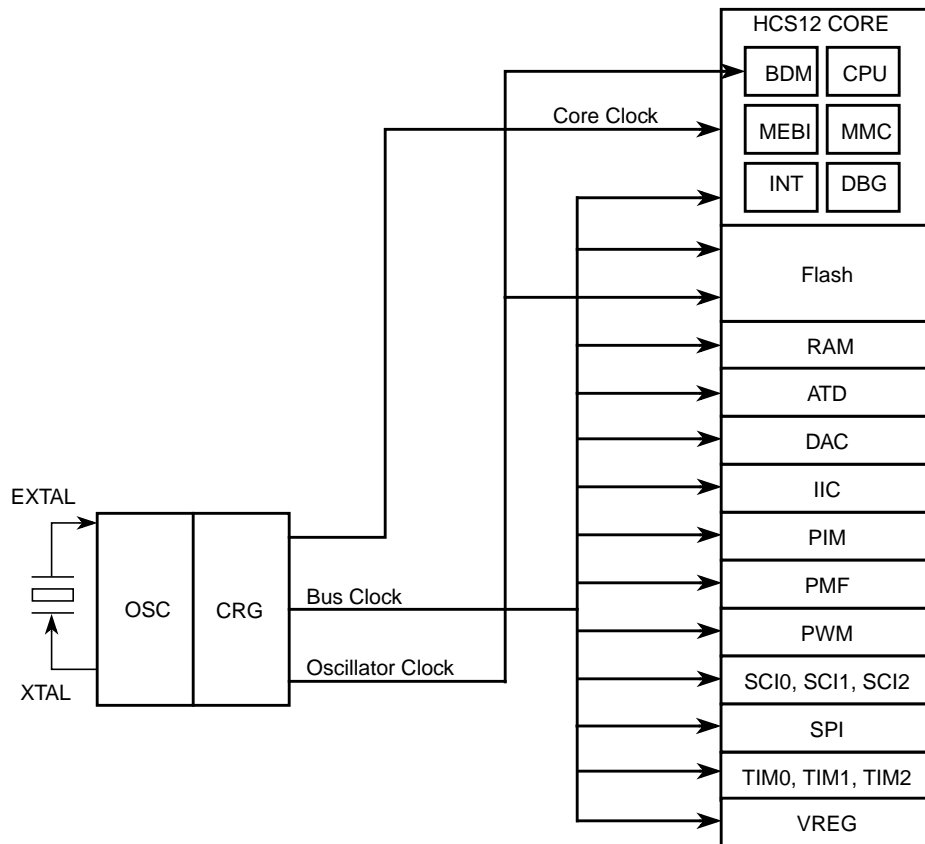
Figure 1-7. Clock Connections
