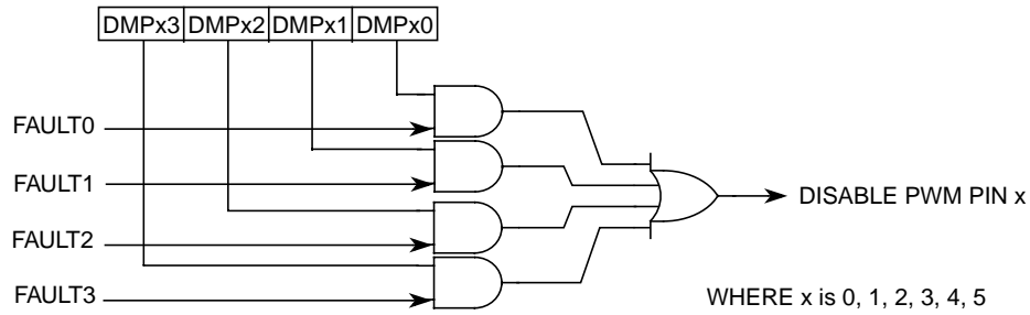
Figure 11-15. Fault Decoder
