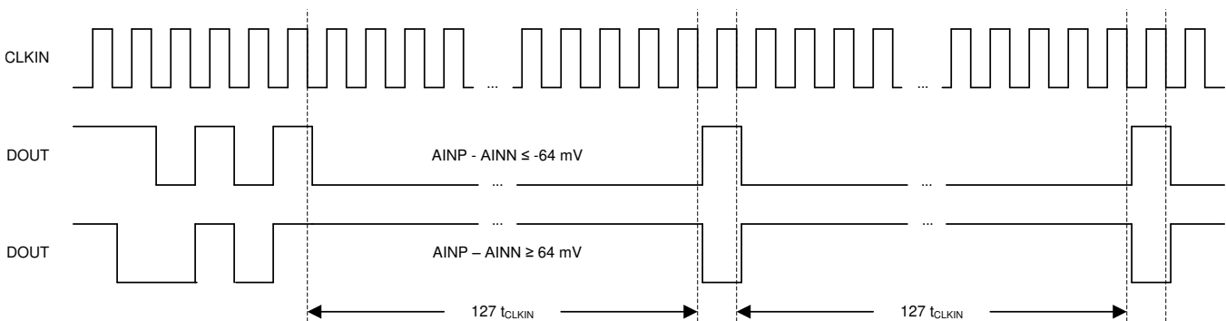
Figure 48. Overrange Output of the AMC1106
