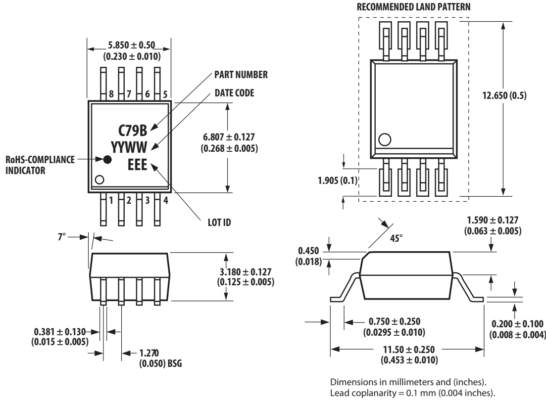
Figure 2: SSO-8 Package
