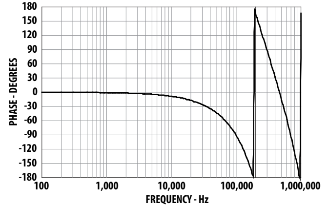
Figure 18: Phase Frequency Response
