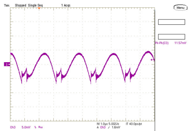
Output Ripple and Noise (Vin=12.0V, Vout=1.8V, Iout=30A, Load=760uF, Scope BW=20MHz)
