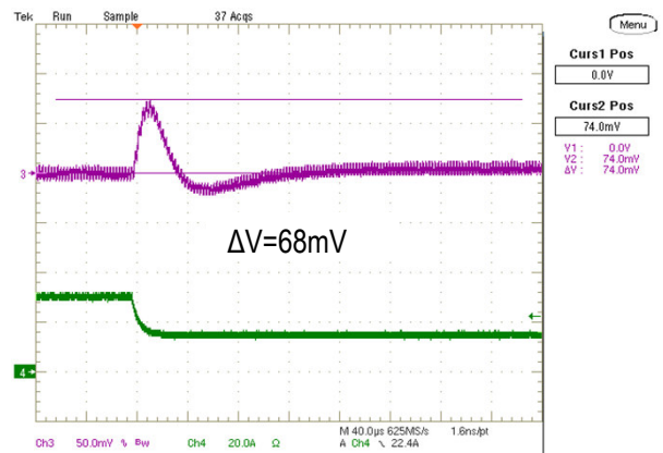
Step Load Transient Response (Vin=12.0V, Vout=1.8V, Load=760uF, Iout=30 to 15A, 1.0A/us) Trace 3=Vout, 50mV/div, Trace 4=Iout, 20A/div.
