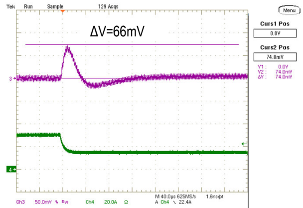
Step Load Transient Response (Vin=5.0V, Vout=1.8V, Cloud=760uF, Iout=30 to 15A, 1.0A/us) Trace 3=Vout, 50mV/div, Trace 4=Iout, 20A/div.
