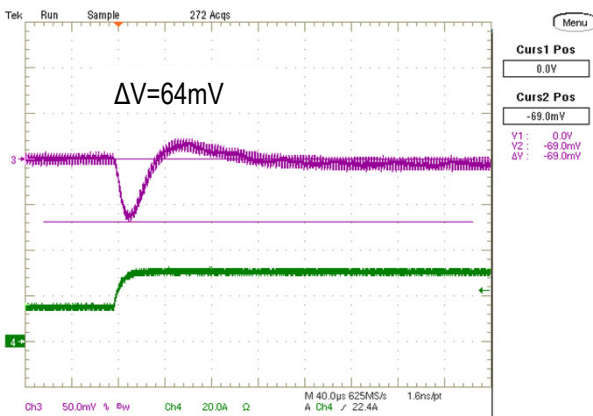
Step Load Transient Response (Vin=12.0V, Vout=1.8V, Load=760uF, Iout=15 to 30A, 1.0A/us) Trace 3=Vout, 50mV/div, Trace 4=Iout, 20A/div.
