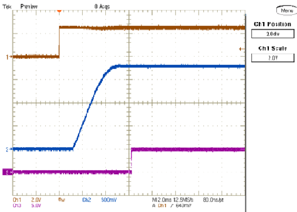
On/Off Enable Delay (Vin=5.0V, Vout=1.8V, Iout=30A, Cloud=760uF) Trace1=Enable, Trace2=Vout, Trace3=P.G
