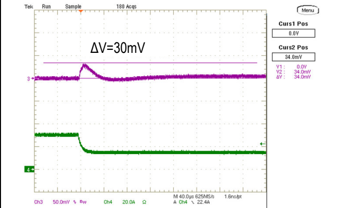
Step Load Transient Response (Vin=12.0V, Vout=0.7V, Cload=760uF, Iout=30 to 15A, 1.0A/us) Trace 3=Vout, 50mV/div, Trace 4=Iout, 20A/div.
