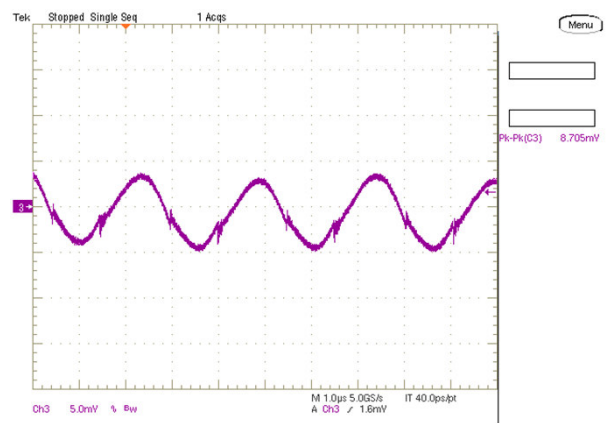
Output Ripple and Noise (Vin=5.0V, Vout=1.8V, Iout=30A, Cloud=760uF, Scope BW=20MHz)
