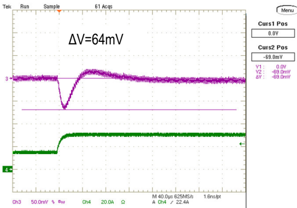
Step Load Transient Response (Vin=5.0V, Vout=1.8V, Cloud=760uF, Iout=15 to 30A, 1.0A/us) Trace 3=Vout, 50mV/div, Trace 4=Iout, 20A/div.
