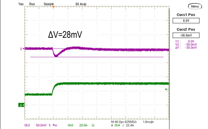
Step Load Transient Response (Vin=12.0V, Vout=0.7V, Cload=760uF, Iout=15 to 30A, 1.0A/us) Trace 3=Vout, 50mV/div, Trace 4=Iout, 20A/div.
