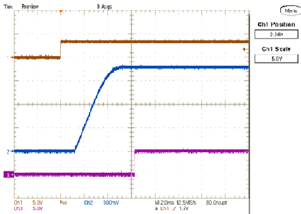
On/Off Enable Delay (Vin=12.0V, Vout=1.8V, Iout=30A, Load=760uF) Trace1=Enable, Trace2=Vout, Trace3=P.G
