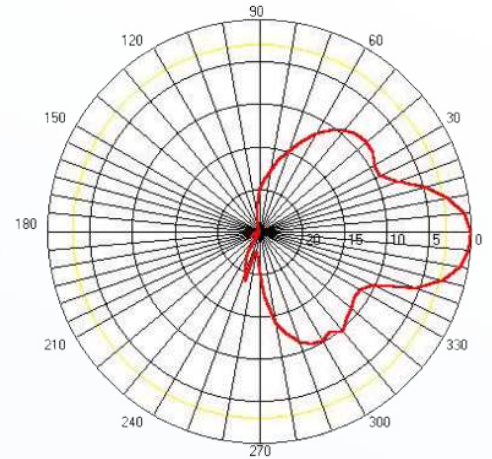
ES24-14 H-Plane at 2.4 GHz
