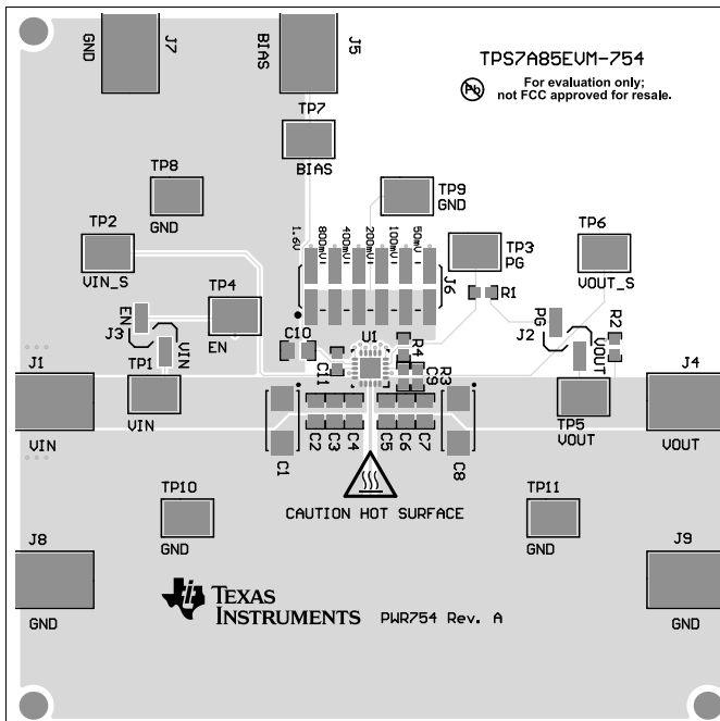
Figure 1. Assembly Layer
