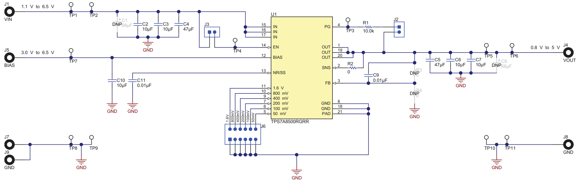
Figure 6. TPS7A85EVM-754 Schematic
