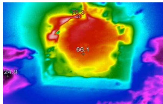
Figure 8. The Two Images Show the LTM4636-1 Operating at 1V at 40A and 3.3V at 35A from a 12V Input. Both Images Reflect Only a 40^\circ\text{C} to 45^\circ\text{C} Rise Above Ambient at Full Load Current with 200LFM
