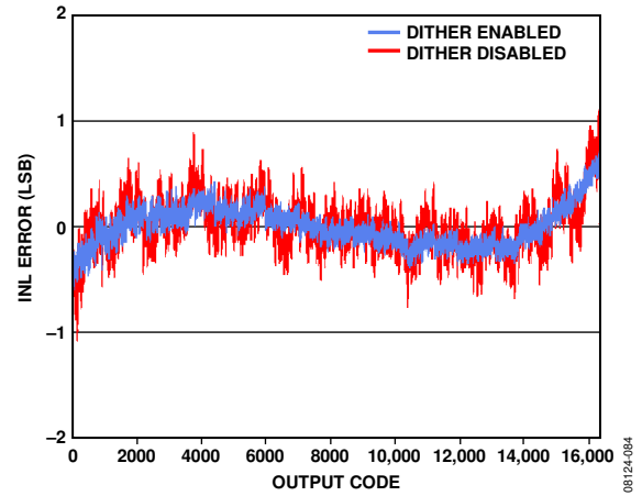
Figure 30. AD9258-105 INL with f_{IN} = 9.7 MHz
