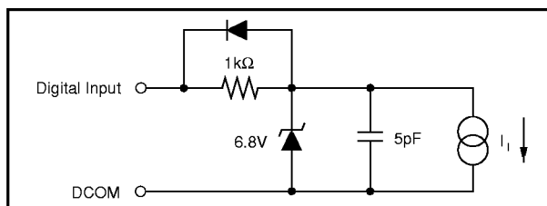
FIGURE 1. Equivalent Digital Input Circuit.
