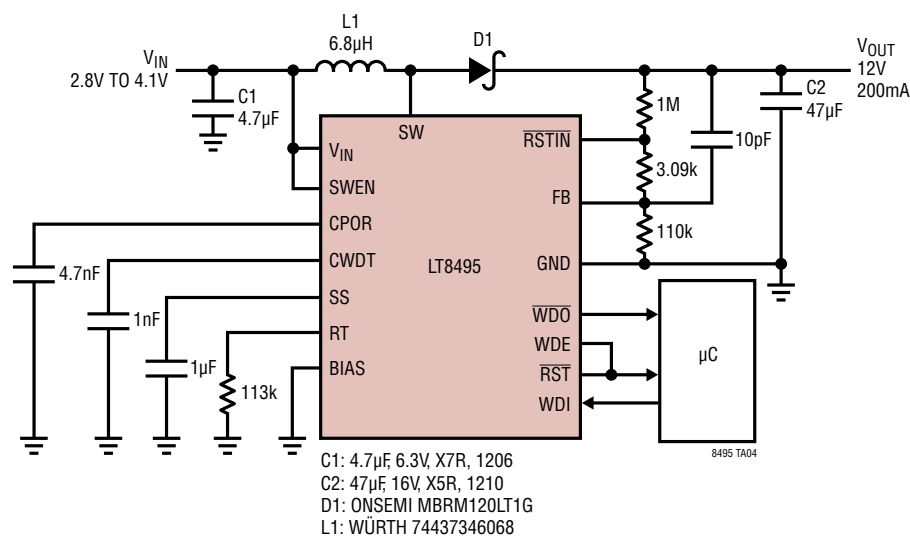
Li-Ion to 12V, Low Q Current Boost @ 650kHz
