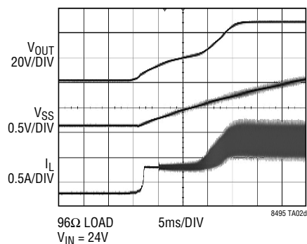
Start-Up Waveforms
