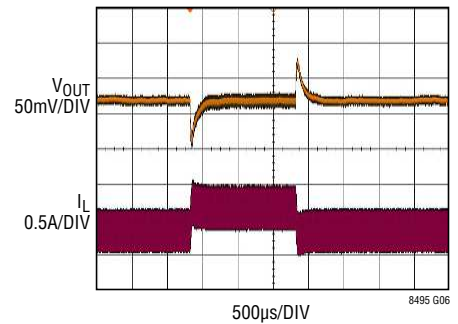
Transient Load Response; Load Current Is Stepped from 300mA to 500mA
