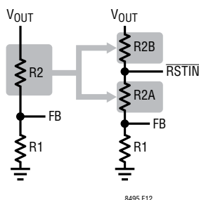
Figure 12. \overline{\text{RSTIN}} Pin Connection Options
