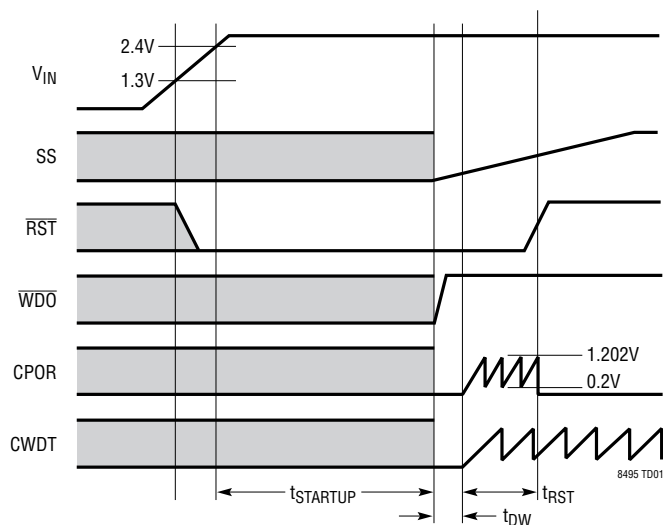
Start-Up Timing
