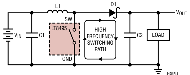
Figure 13. High Speed Chopped Switching Path for Boost Topology
