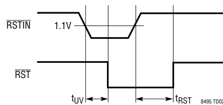
RSTIN Timing
