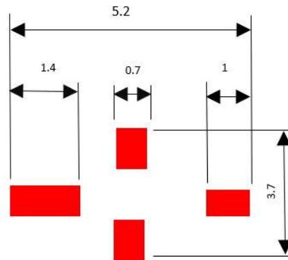
PCB Footprint
