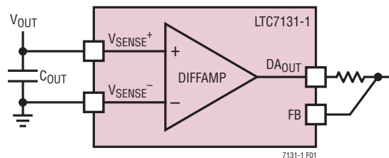
Figure 1. Differential Amplifier Connection
