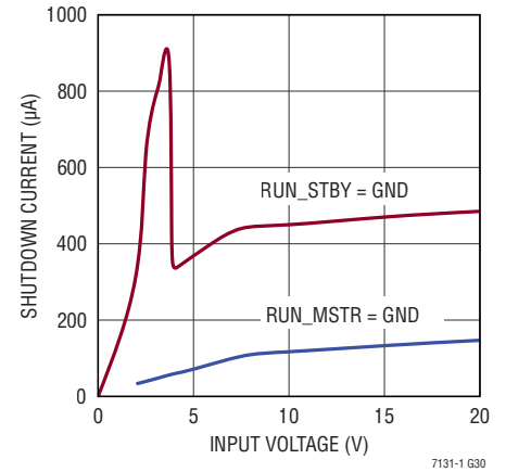
Standby Current vs Input Voltage
