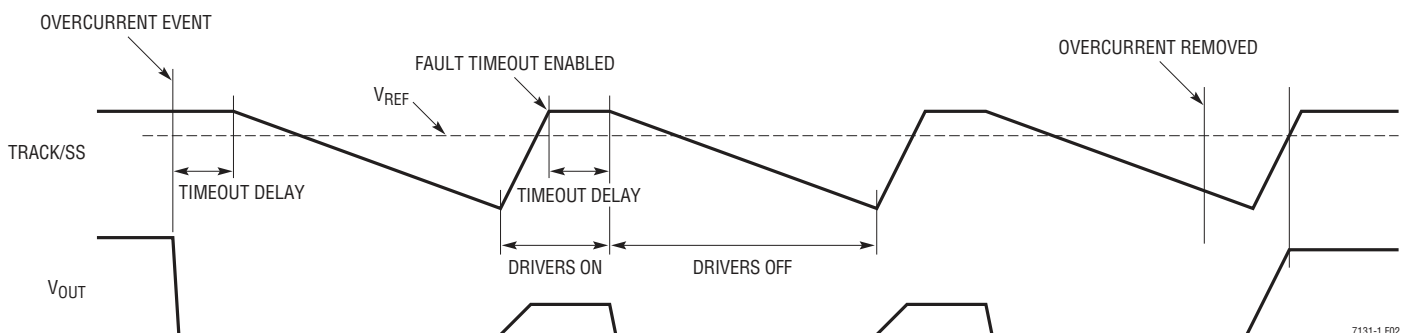
Figure 2. Fault Response Timing to Overcurrent Event
