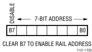
Figure 23. MFR_RAIL_ADDRESS Data Byte
