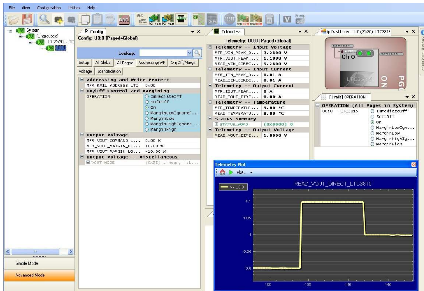
Figure 22. LTPowerPlay
