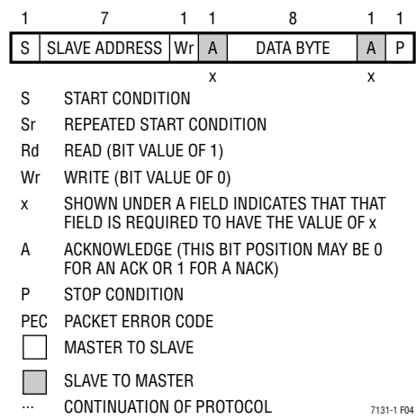
Figure 4. PMBus Packet Protocol Diagram Element Key
