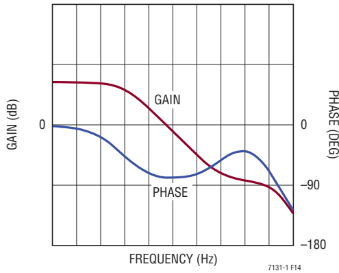
Figure 14. Transfer Function of Buck Modulator
