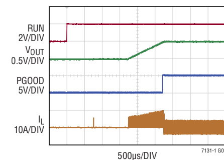
Start-Up Into Prebiased Output
