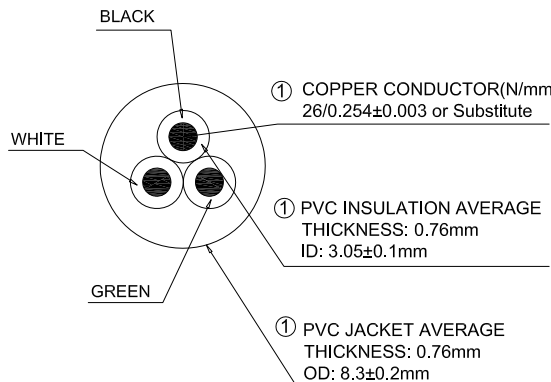
Wire cross section
