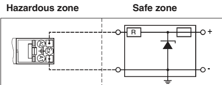
Sub-base for intrinsic safety miniature solenoid valve
