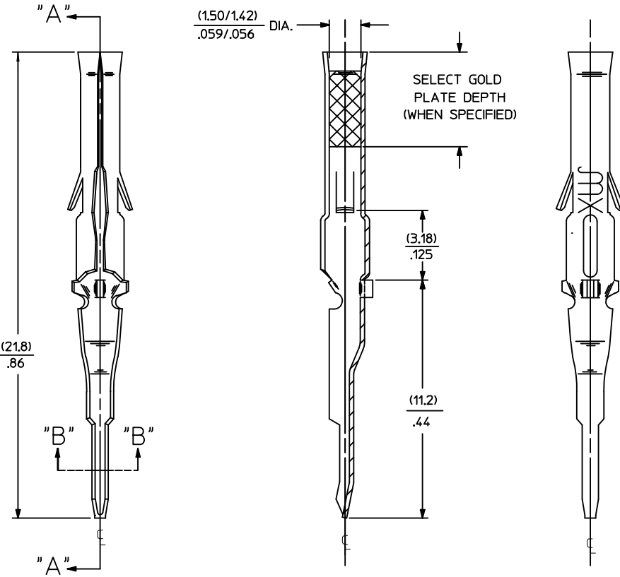
SECT. "A-A"
