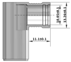
Detail A-A Sizes E, A, B, C and D
