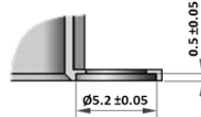
Detail B-B
