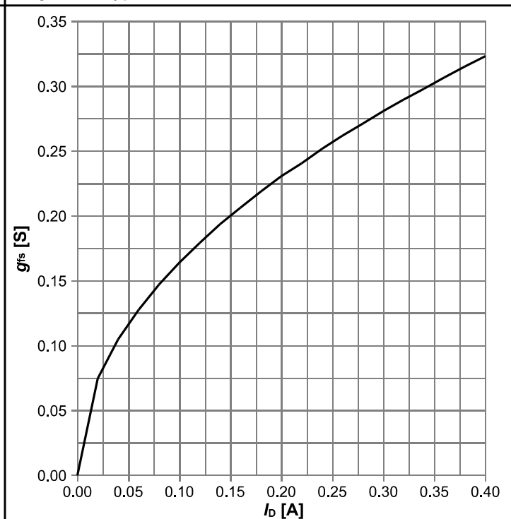
Diagram 8: Typ. transconductance
