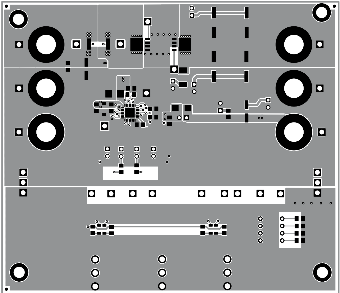
Figure 6. Top Layer Routing
