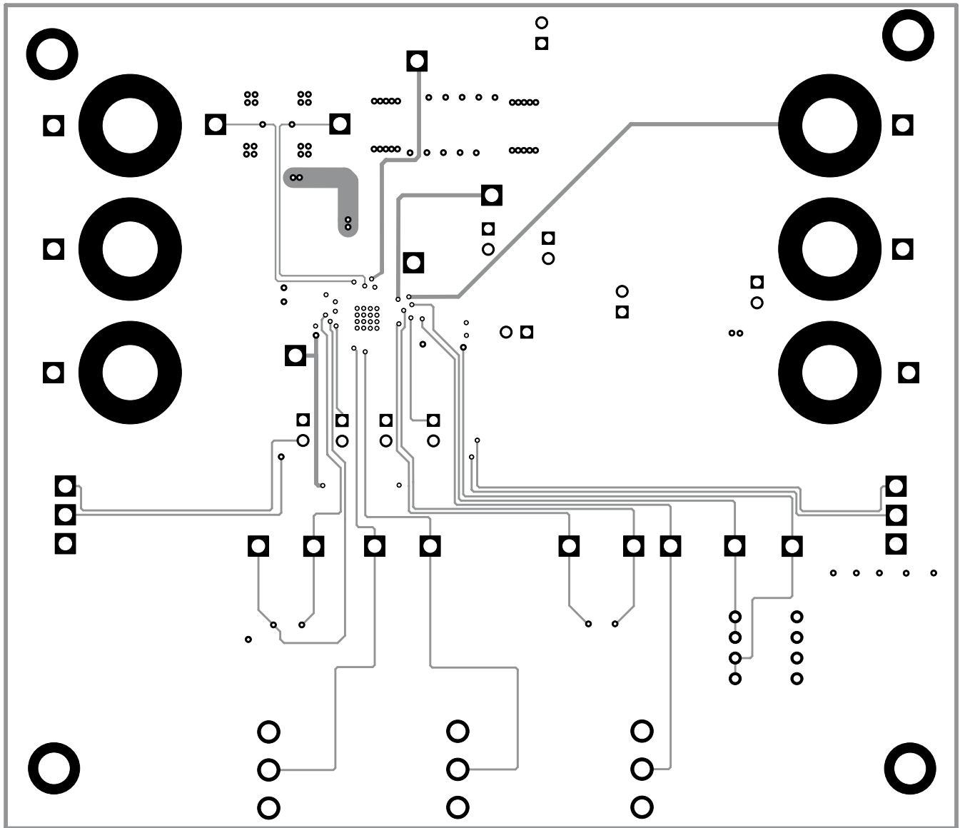
Figure 8. Layer 3 Routing
