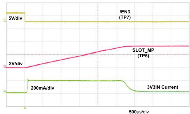
Figure 4. Output Ramp-Up Waveforms – SLOT_MP Rail
