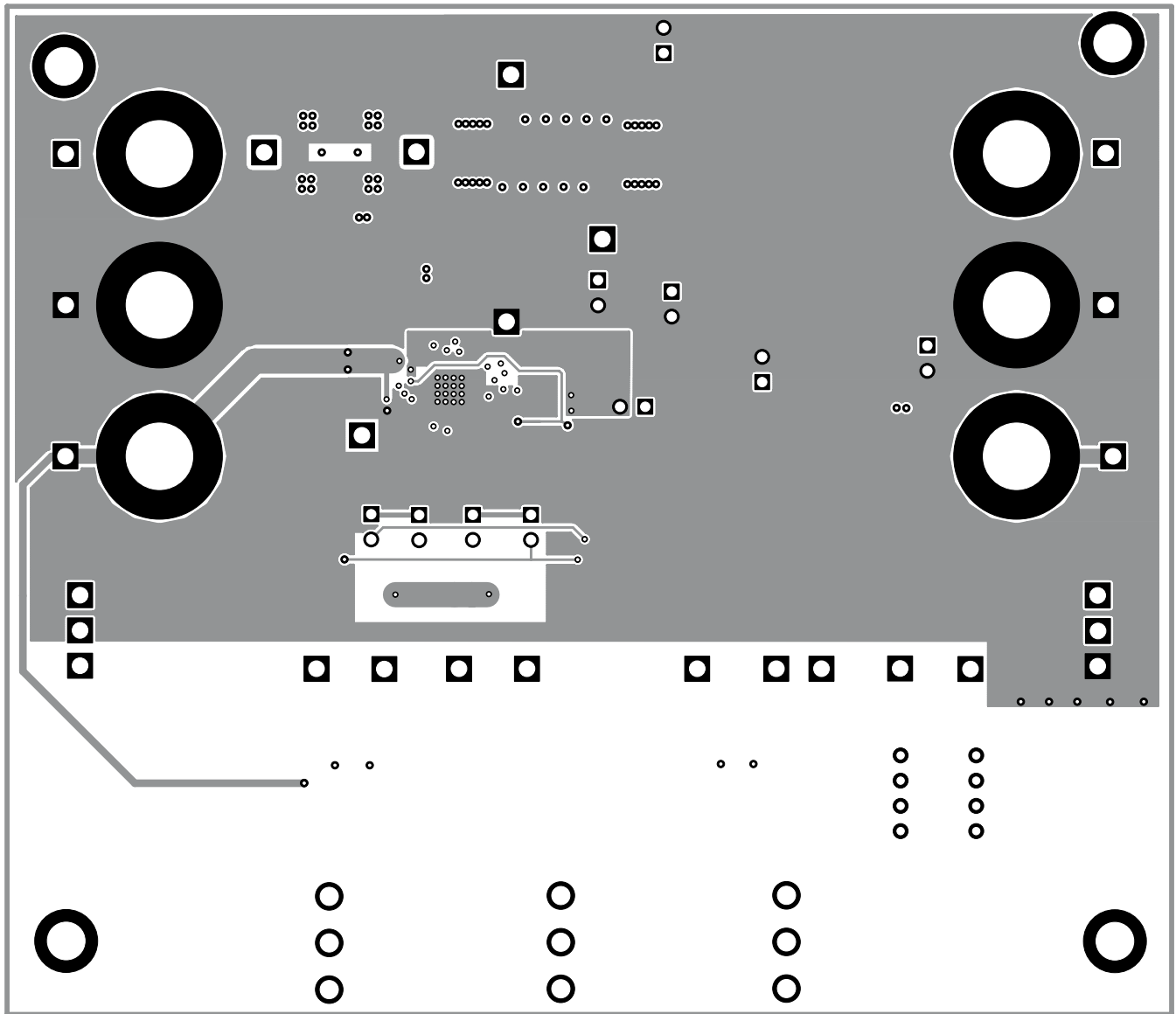
Figure 7. Layer 2 Routing
