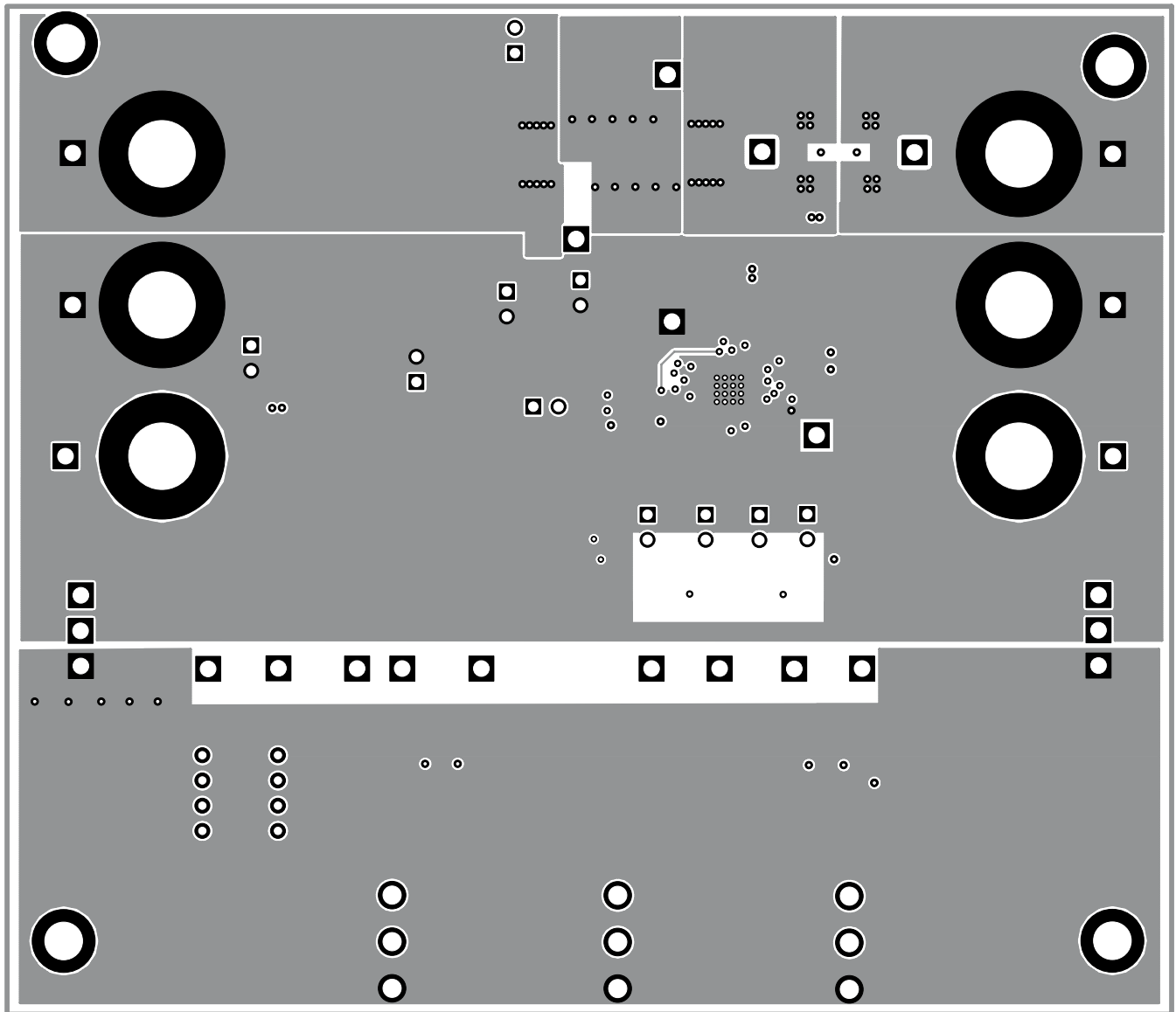
Figure 9. Bottom Layer Routing
