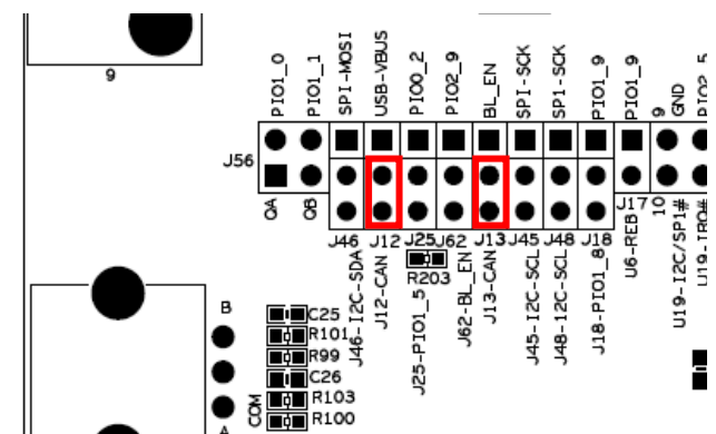
Figure 52 – Jumper Setting: CAN, U4
