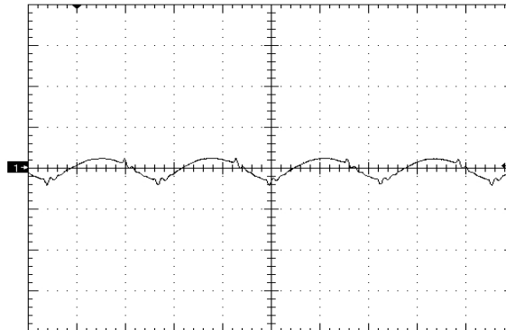
Figure 8. Output Voltage Ripple (50mV/div), time scale – 1uS/div. Vin=Vin_nom, full load Cout=1uF ceramic + 10uF Tantalum (see Fig 16)
