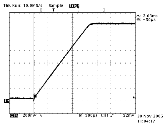
Figure 34. AMD Startup
