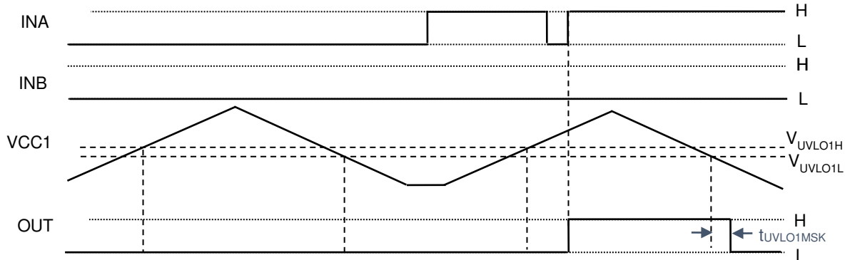
Figure 4. Timing Chart of Input-side UVLO Function
