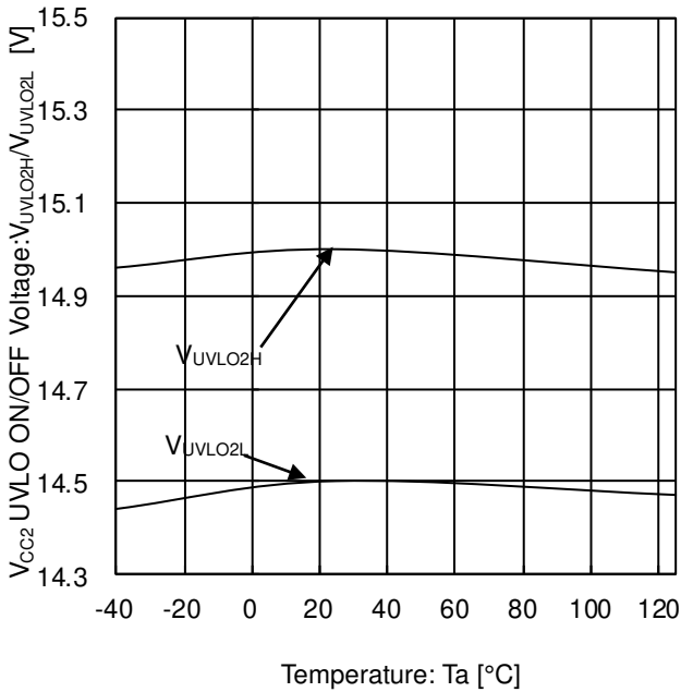
Figure 29. V CC2 UVLO ON/OFF Voltage vs Temperature
