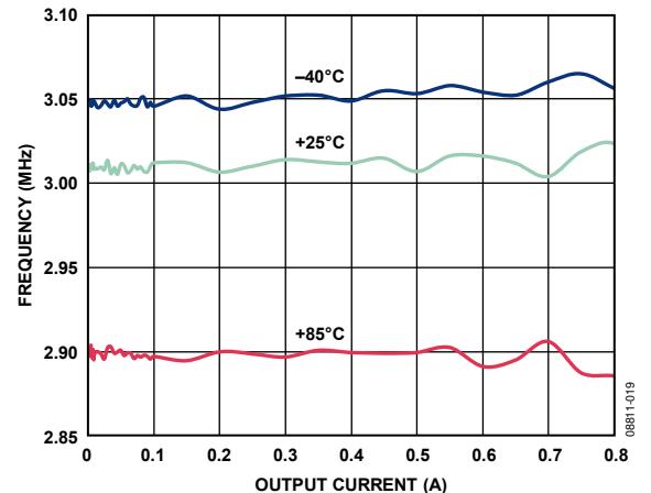
Figure 19. Buck Switching Frequency vs. Output Current, Across Temperature, V_{OUT1} = 1.8\text{ V} , PWM Mode
