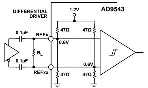
Figure 29. Differential AC-Coupled Mode ( R_L = 100 \Omega Is Recommended, Except For HCSSL)
