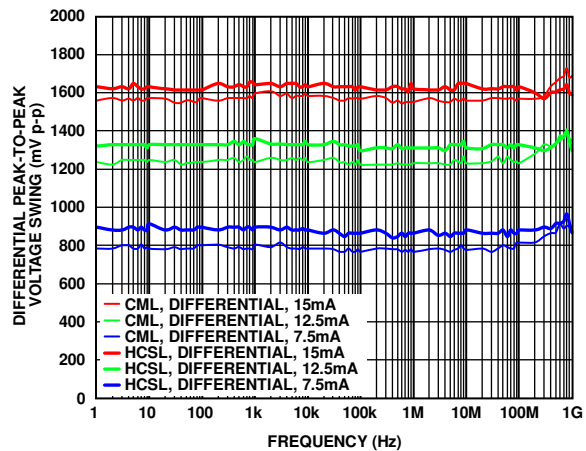
Figure 20. Differential Output Amplitude Waveforms; HCSL Drivers Terminated 50 Ω to GND per Figure 32; CML Drivers Terminated 50 Ω to 1.8 V per Figure 33
