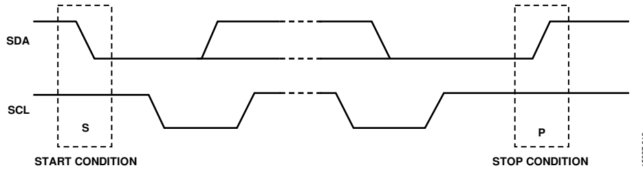
Figure 61. Start and Stop Conditions
