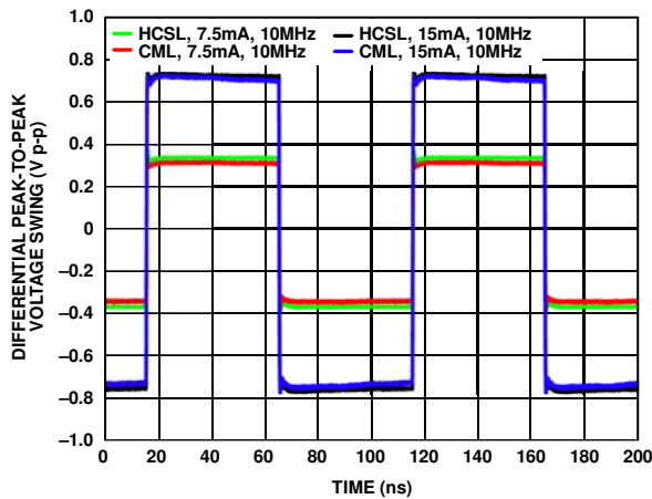
Figure 17. 10 MHz Output Waveforms for Various Driver Settings; HCSL Drivers Terminated 50 Ω to GND per Figure 32; CML Drivers Terminated 50 Ω to 1.8 V per Figure 33
