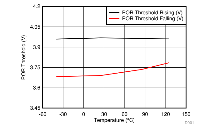
Figure 1. POR Threshold ( V_{POR} ) vs Temperature
