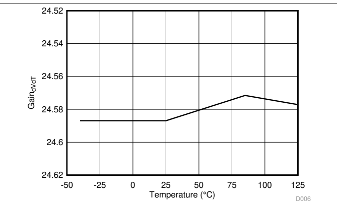
Figure 6. GAIN_{(dVdT)} vs Temperature
