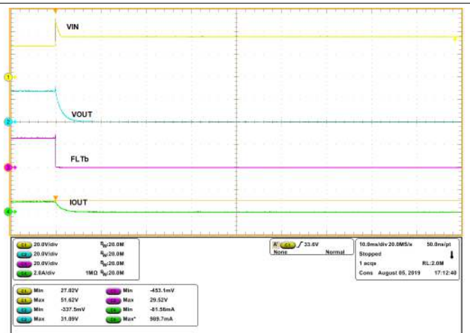
Figure 22. OVP Overvoltage Cut-Off
