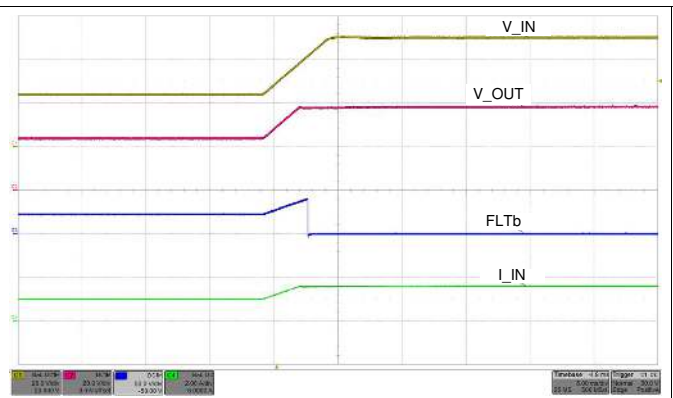
Figure 26. Internal OV Clamp Response
