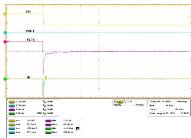
Figure 46. Protection from Reverse Battery [ V_{IN} = -24 V, V_{OUT} = 0 V, I_{LIM} = 2.23 A]
